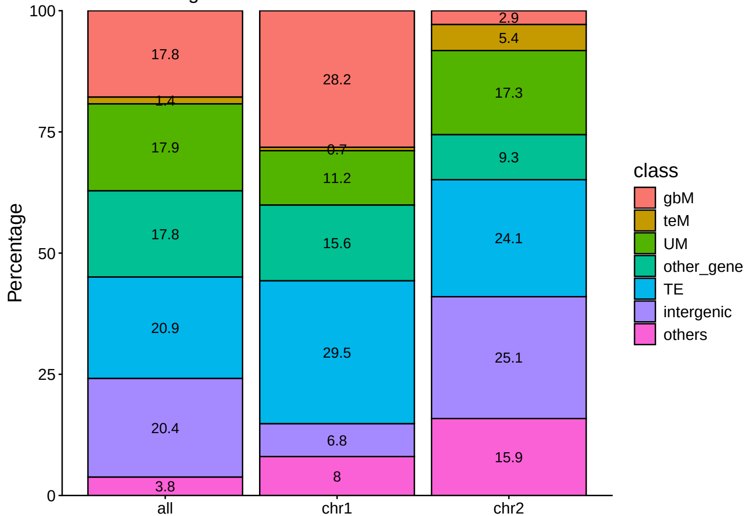
global 5kb window chr1 chr2 trans
